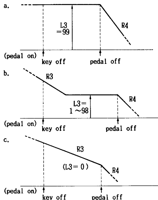
PITCH EG (fig. 36)
