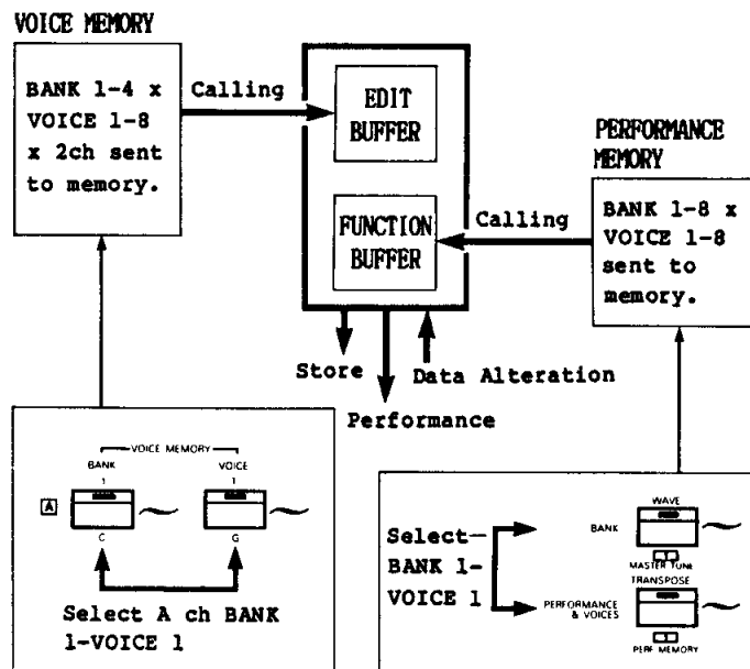
Fig.10. Buffer Circuitry
