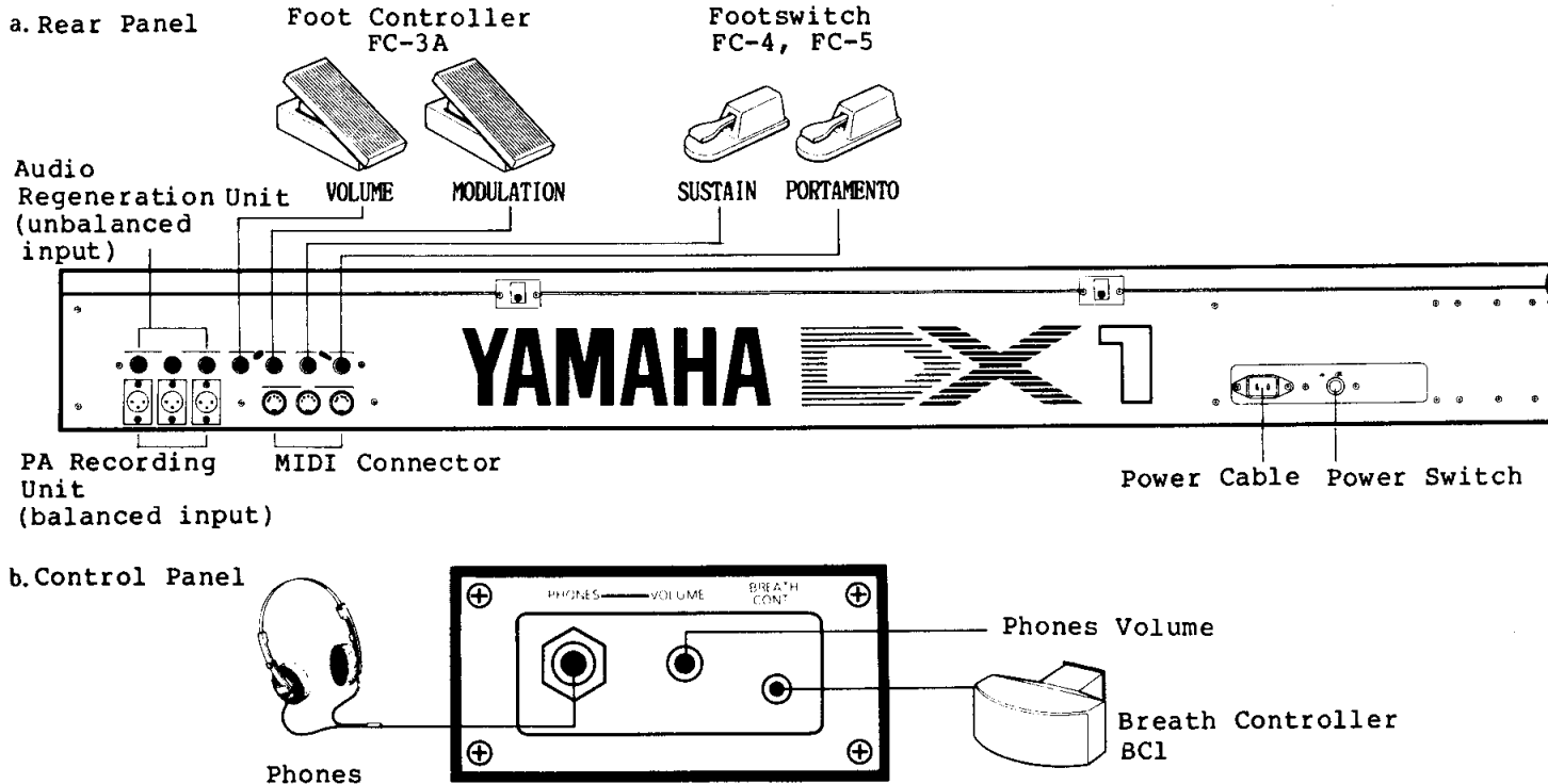
Fig. 9. Connection Terminals
